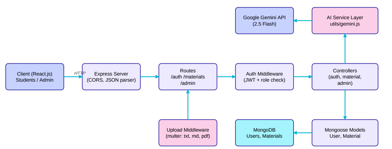
Figure 1: AI StudyBuddy architecture and data flow
